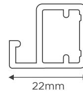
AP-64 Finish : Anodised, BS Make : Virgin Aluminium Description : Frame Profile for 4mm glass
