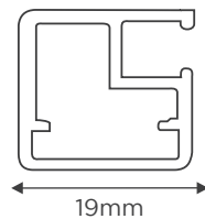
AP-40 Finish : Anodised, SS, BS Make : Virgin Aluminium Description : Frame Profile for 4mm glass
